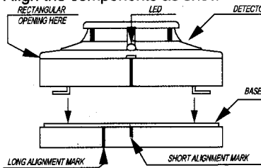
Fig.2 Mating detector head onto base
