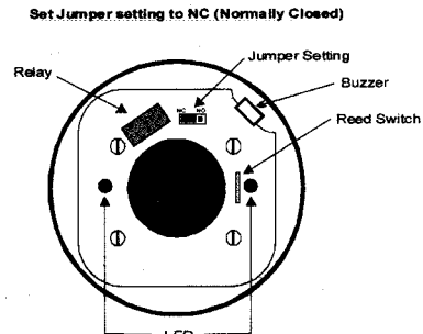
Fig. 4 Schematic of detector Structure When front cover is open.
