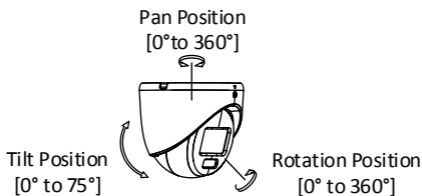
Figure 2-27 3-Axis Adjustment
