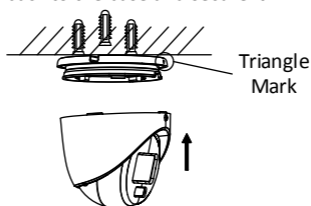
Figure 2-26 Install the Camera Back
