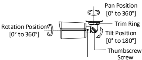
Figure 2-10 3-Axis Adjustment
