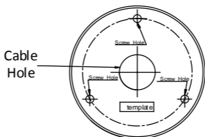
Figure 2-8 Drill Template
