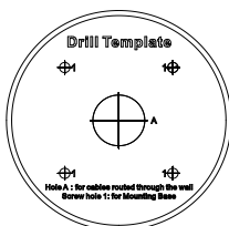
Figure 2-5 Drill Template of the Junction Box
