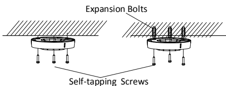
Figure 2-2 Attach the Mounting Base to the Ceiling
