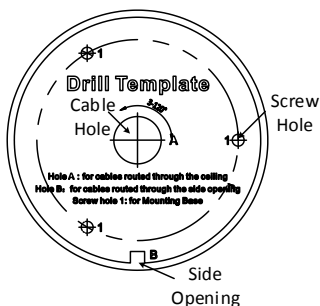
Figure 2-1 Drill Template
