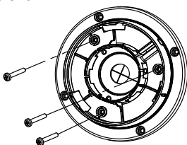
Figure 2-6 Install Turret Camera's Mounting Base
