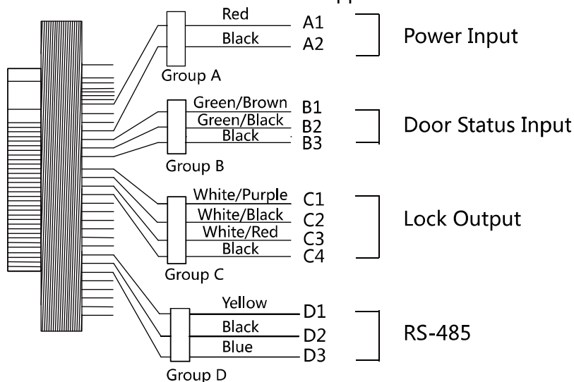
Figure 3. 1 Terminals Diagram
