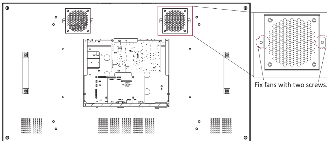
Figure 2-5 Fix Fans
