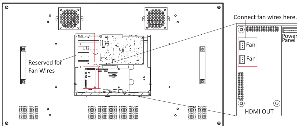
Figure 2-4 Connect Fan Wires
