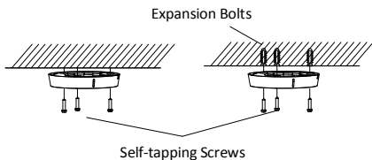
Figure 2-10 Attach the Mounting Base to the Ceiling
