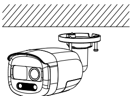
Figure 2-2 Attach the Camera to the Ceiling
