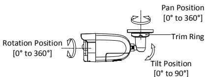
Figure 2-3 3-Axis Adjustment
