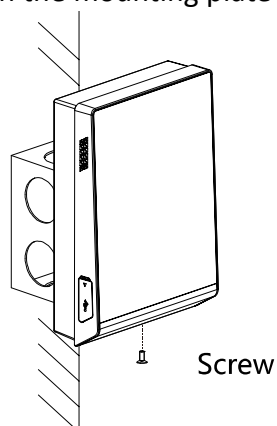
Figure 3-4 Tighten Screw
