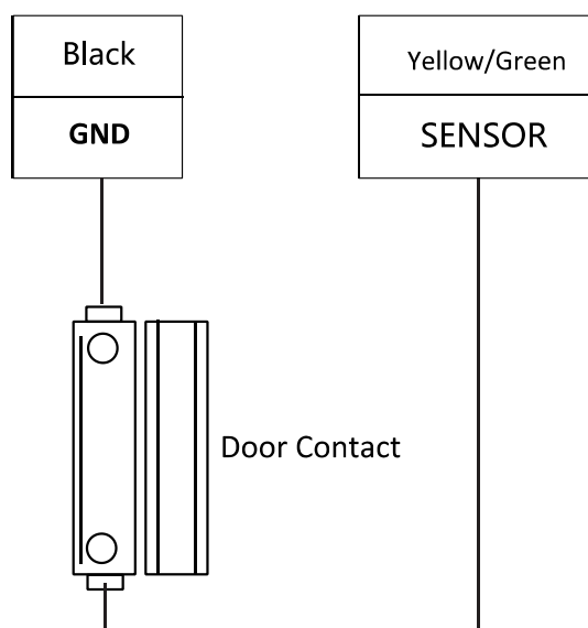
Figure 5-5 The Installation of Door Contact
