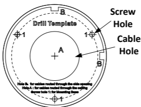
Figure 2. 1 Drill Template
