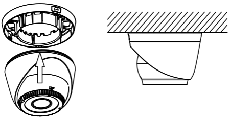
Figure 2. 7 Secure the Camera with Mounting Base
