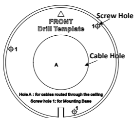
Figure 2. 4 Drill Template
