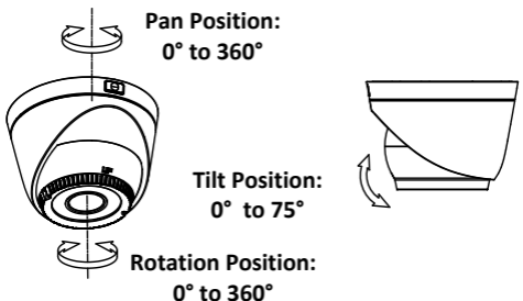
Figure 2. 8 3-axis Adjustment
