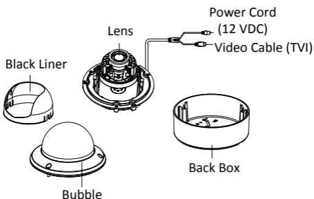
Figure 1. 3 Type III Camera Overview
