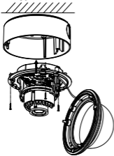
Figure 2. 11 Fix the Camera to the Ceiling
