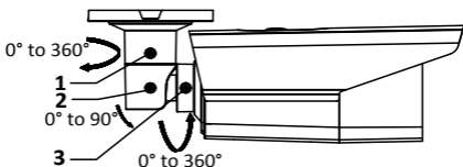
Figure 2. 3 3-Axis Adjustment
