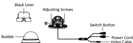
Figure 1-10 Overview of Type VI Camera (with F)
