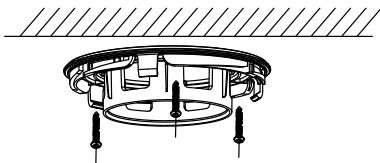
Figure 2-5 Secure the Mounting Base
