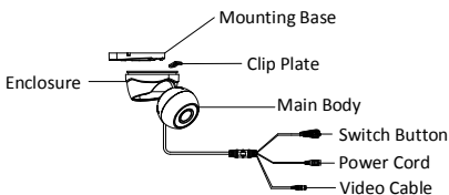
Figure 1-2 Overview of Type I Camera (with F)
