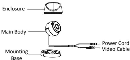
Figure 1-5 Overview of Type III Camera (without F)
