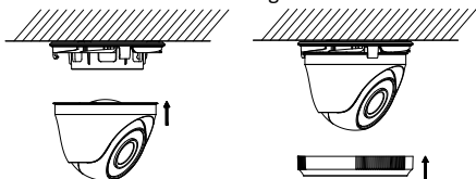
Figure 2-6 Install the Camera back
