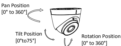
Figure 2-11 3-Axis Adjustment
