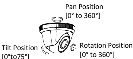
Figure 2-7 3-Axis Adjustment
