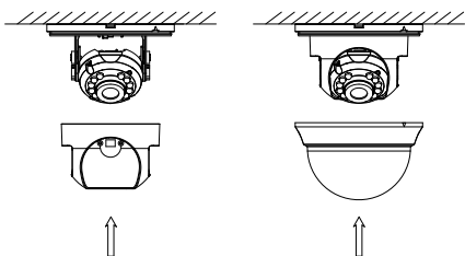
Figure 2-15 Install the Black Liner and the Bubble
