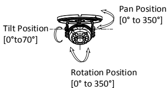
Figure 2-14 3-Aixs Adjustment
