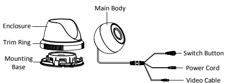
Figure 1-4 Overview of Type II Camera (with F)
