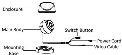
Figure 1-6 Overview of Type III Camera (with F)
