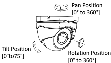
Figure 2-4 3-Axis Adjustment
