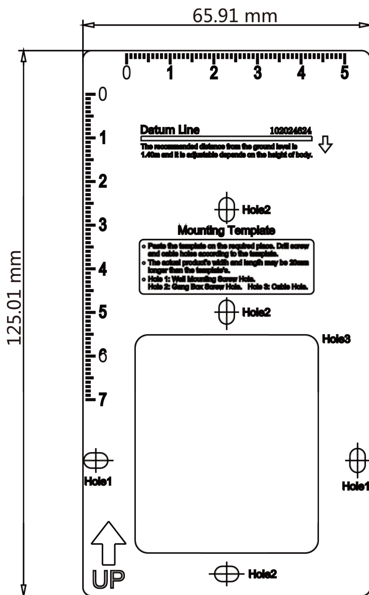
Figure 3-5 Mounting Template
