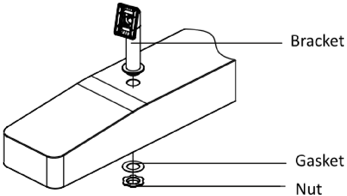
Figure 3-13 Fix Bracket
