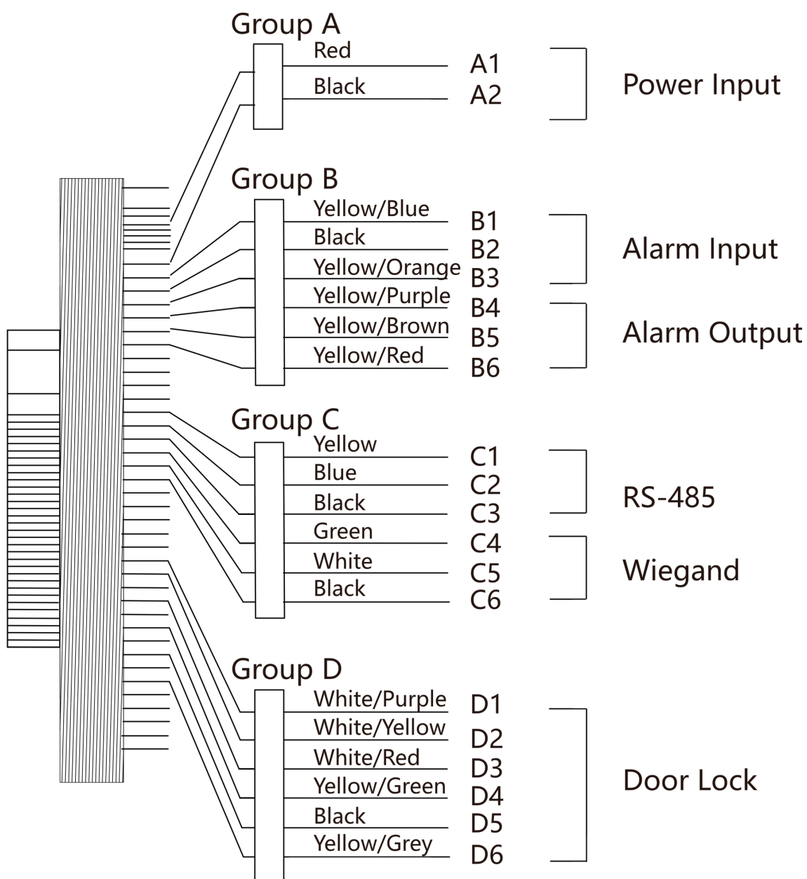
Figure 4-1 Terminal Diagram
