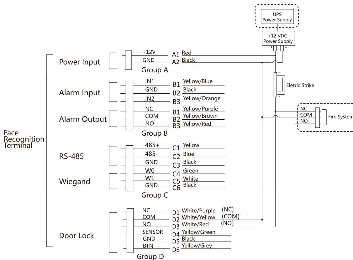
Figure 4-8 Device Wiring
