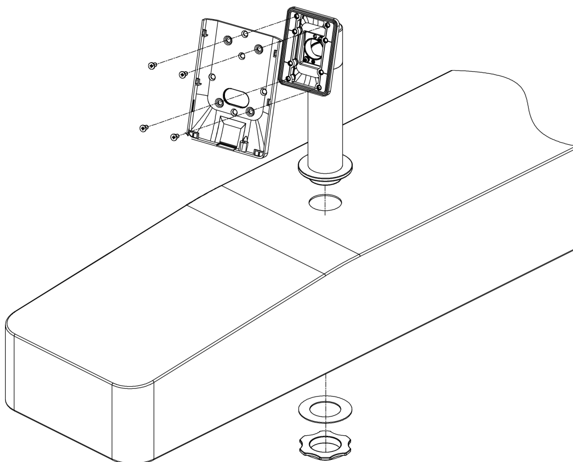
Figure 3-14 Fix Mounting Plate
