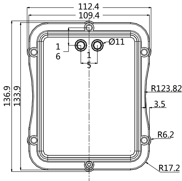
Vista frontal
