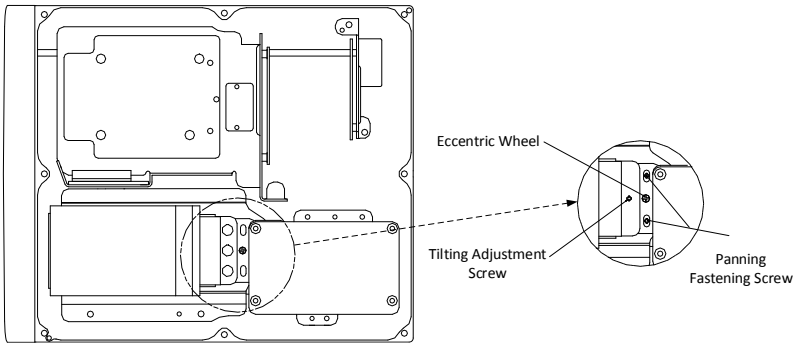
Figure 2-9 Adjust the Laser (Type IV)
