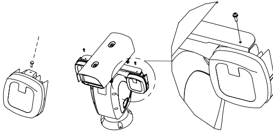
Figure 2-13 Secure the IR Module
