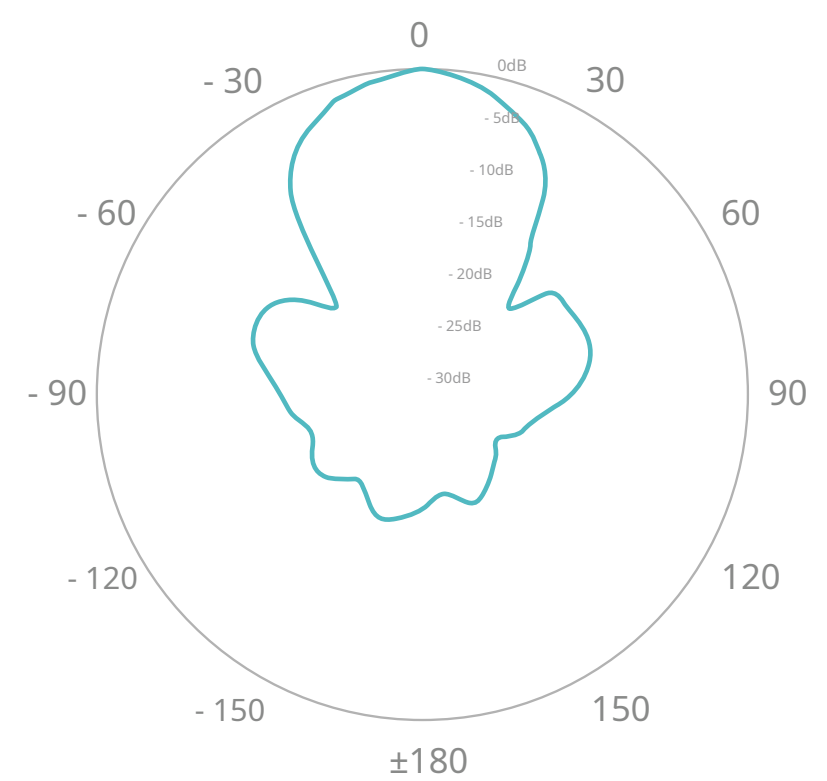
Azimut vertical
