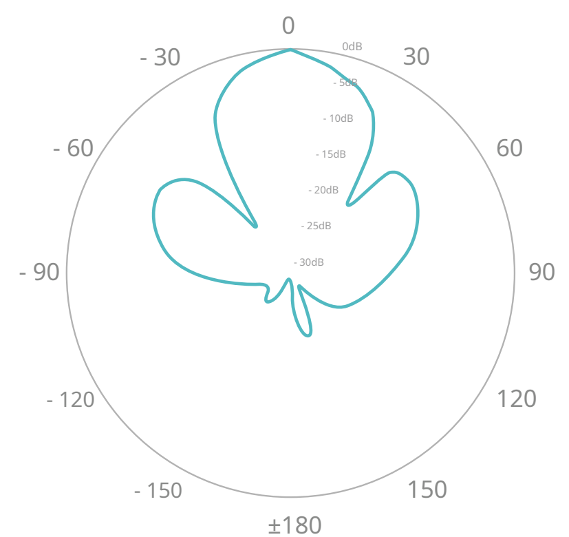
Azimut horizontal
