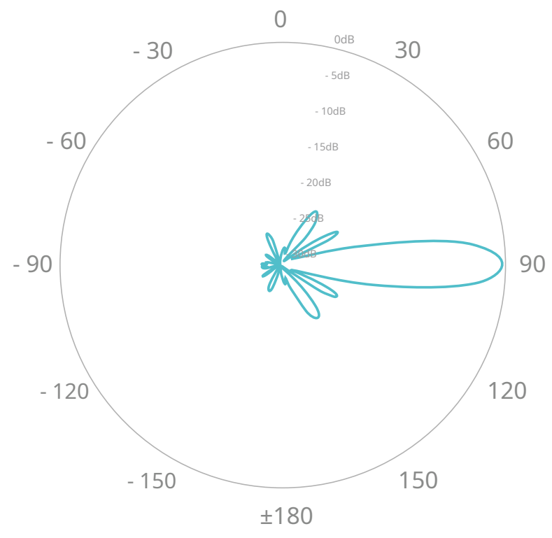
Azimut vertical
