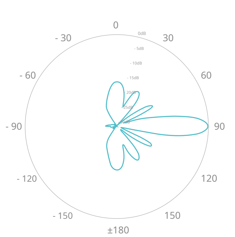
Azimut horizontal
